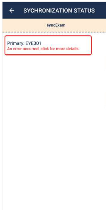
Figure 50: Synchronization details
