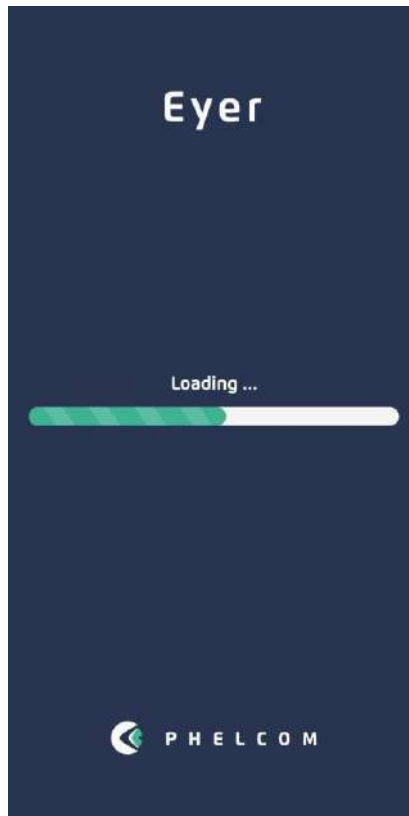
Figure 7: Startup message
