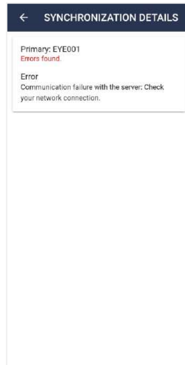
Figure 51: Synchronization status
