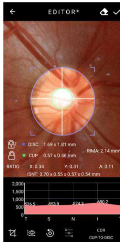
Figure 61: Padlock demonstrate
