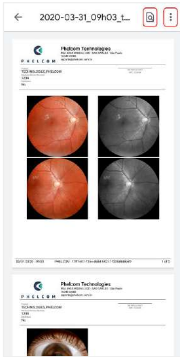
Figure 71: Application-generated report
