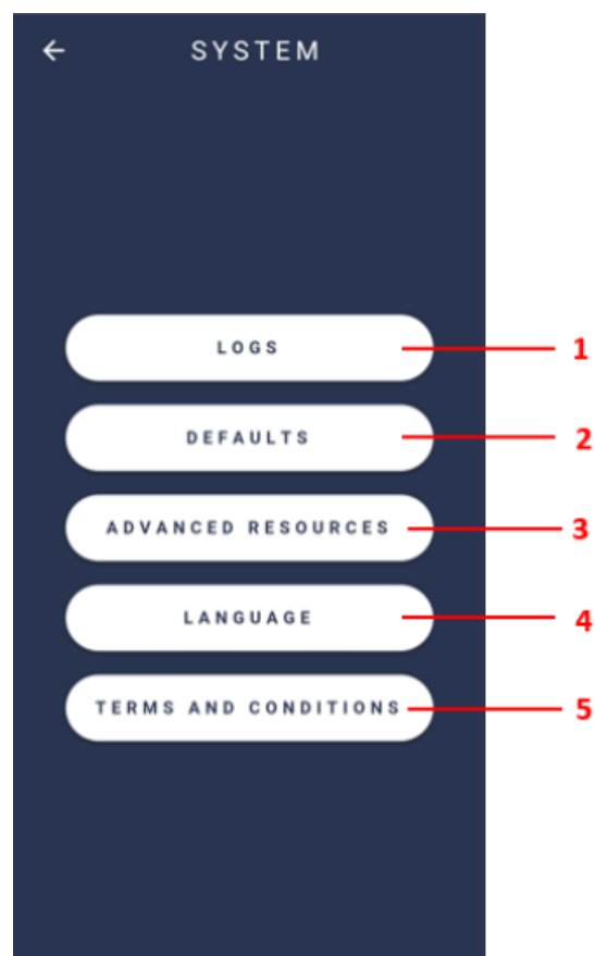
Figure 95: System screen
