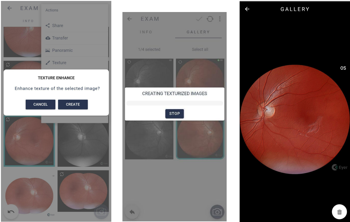
Figure 62: Generate texture
