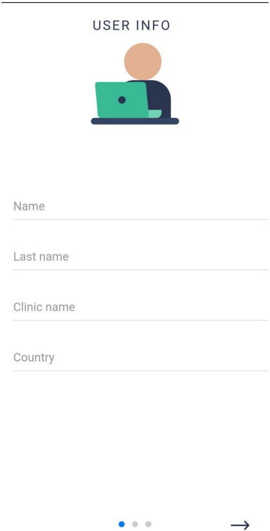
Figure 18 - User Info
