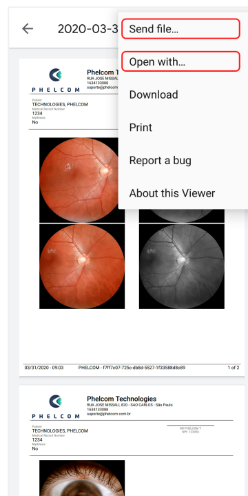
Figure 89: File options
