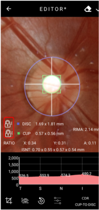
Figure 77: Padlock demonstrate
