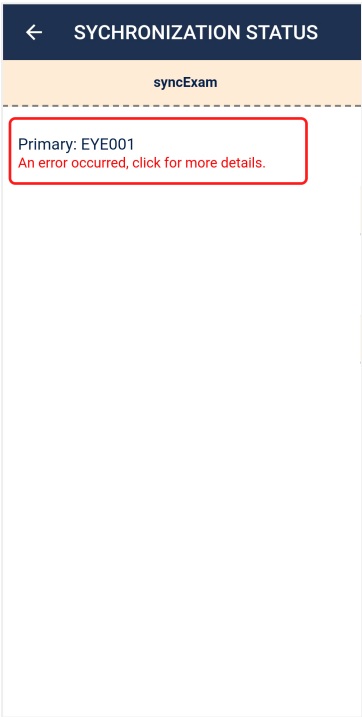
Figure 67: Synchronization details
