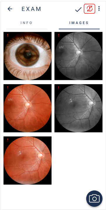
Figure 66: Synchronization failure
