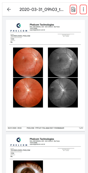
Figure 88: Application-generated report
