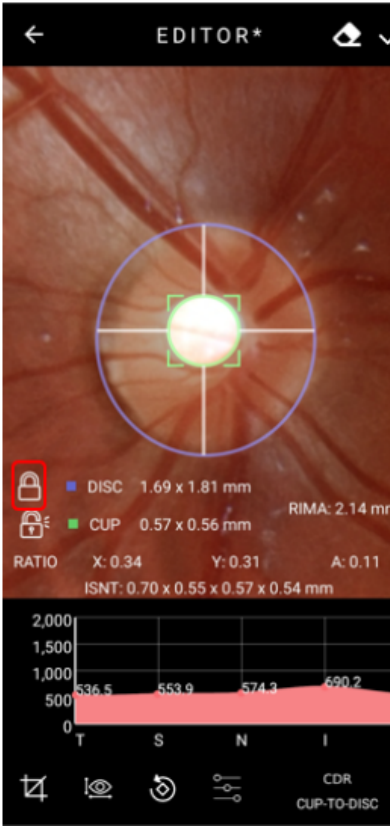
Figure 76: Padlock demonstrate
