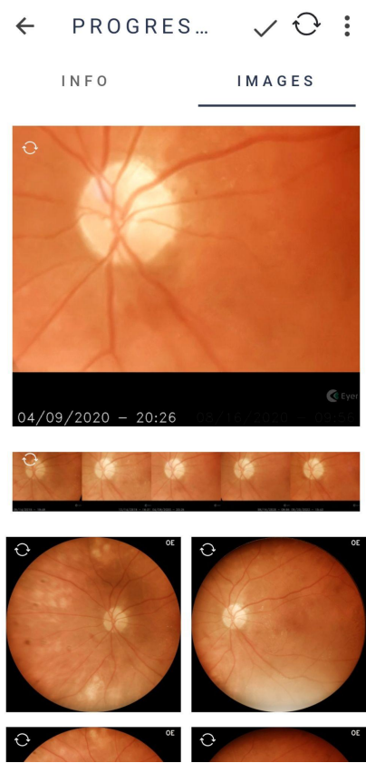
Figure 53: Selection area.
