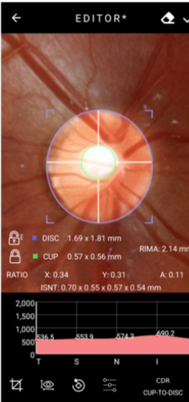
Figure 78: Padlock demonstrate
