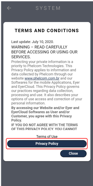
Figure 103: Privacy Policy
