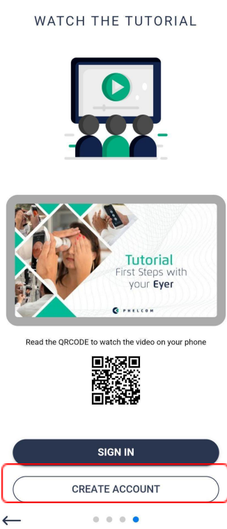
Figure 17 - Create Account
