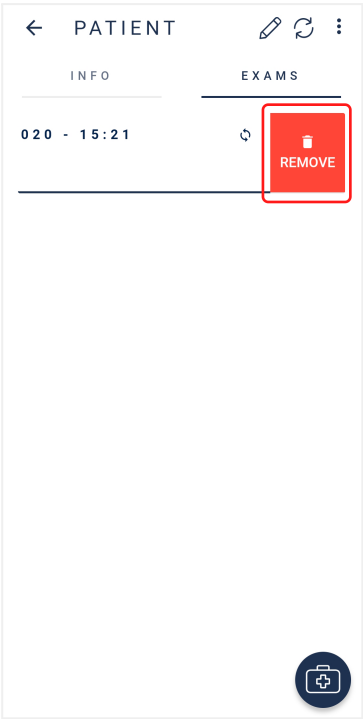
Figure 81: Removing exam
